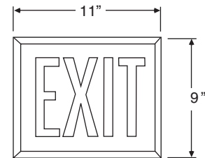
C3-1 AC Only Front View
