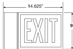
C3-3 Side Mount Housing Front View
