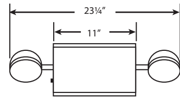
C8-2-24/36 Front View
